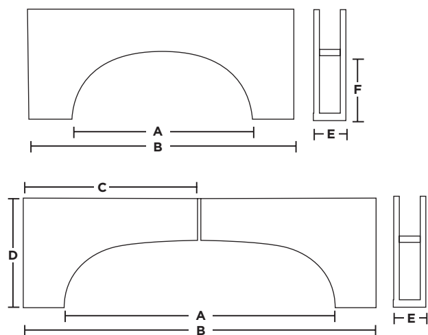
DIMENSIONS (mm)
